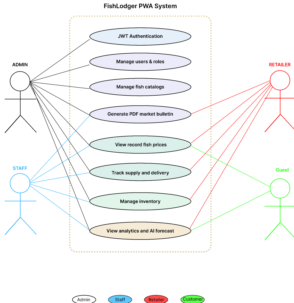
Figure 2. Use Case Diagram for Fishlodger
