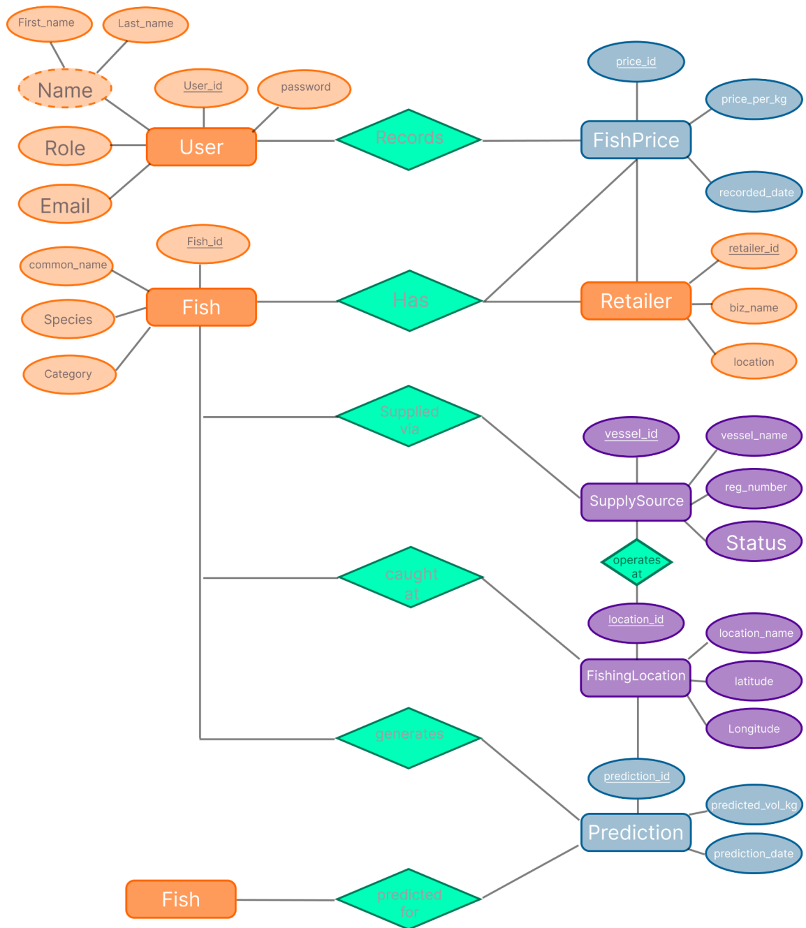
Figure 5. Entity Relationship Diagram
