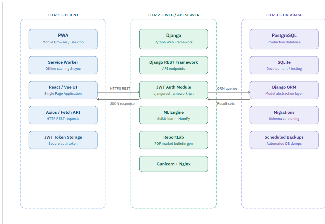
Figure 20. Deployment Diagram
